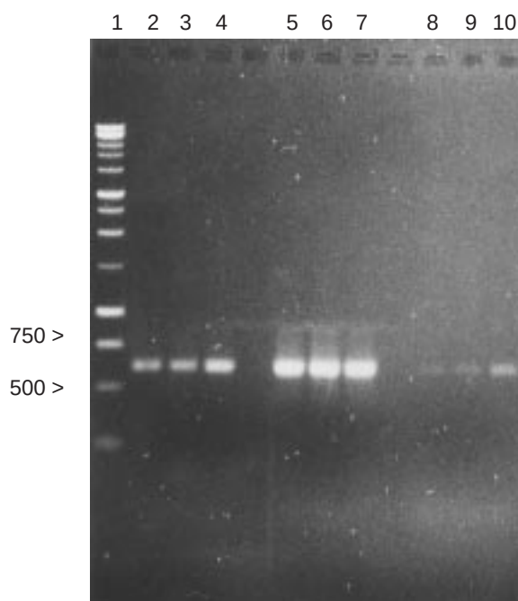
Figure 4. Detection of DNA from Fusarium oxysporum f.sp. ciceris in one artificial and two natural soils using specific wilt-associated, nested primers. DNA extracts were used for PCR after deproteinisation. Three concentrations of skimmed milk were used. Lanes: (1) 1 kb Ladder (Promega); (2–4) artificial soil; (5–7) natural soil A; (8–10) natural soil C; (2,5,8) 3.2% skimmed milk; (3,6,9) 4.0% skimmed milk; (4,7,10) 4.8% skimmed milk.
