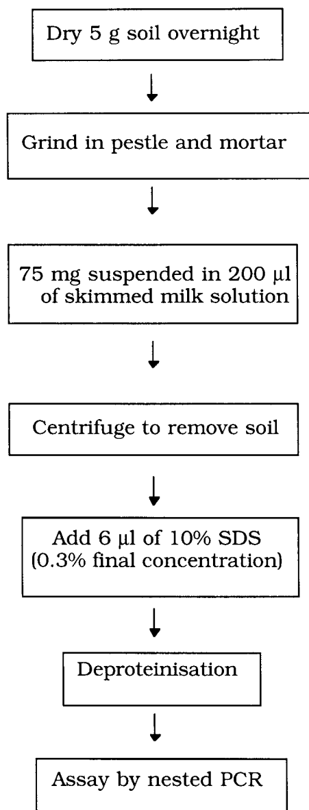
Figure 1. Simplified procedure for extracting fungal DNA from infested soil for detection by PCR.
