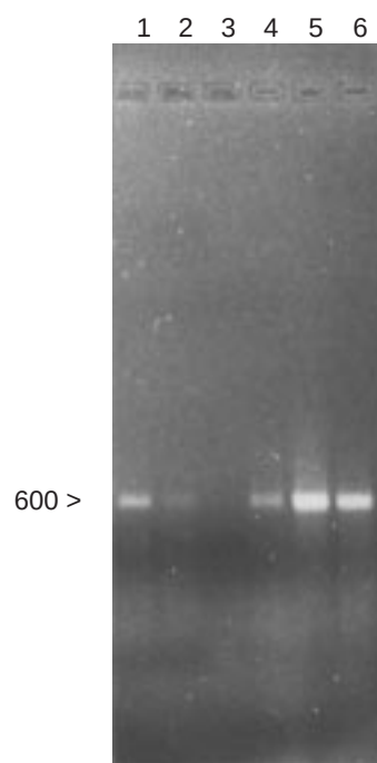
Figure 3. Detection of DNA from Fusarium oxysporum f.sp. ciceris in artificial soil using specific wilt-associated, nested primers. DNA extracts were used for amplification after deproteinisation. Two concentrations of skimmed milk and three volumes of DNA extract were used. Lanes: (1–3) 2.4% skimmed milk; (4–6) 3.2% skimmed milk. (1,4) 1 \mu l DNA extract; (2,5) 2 \mu l soil extract; (3,6) 4 \mu l soil extract.
