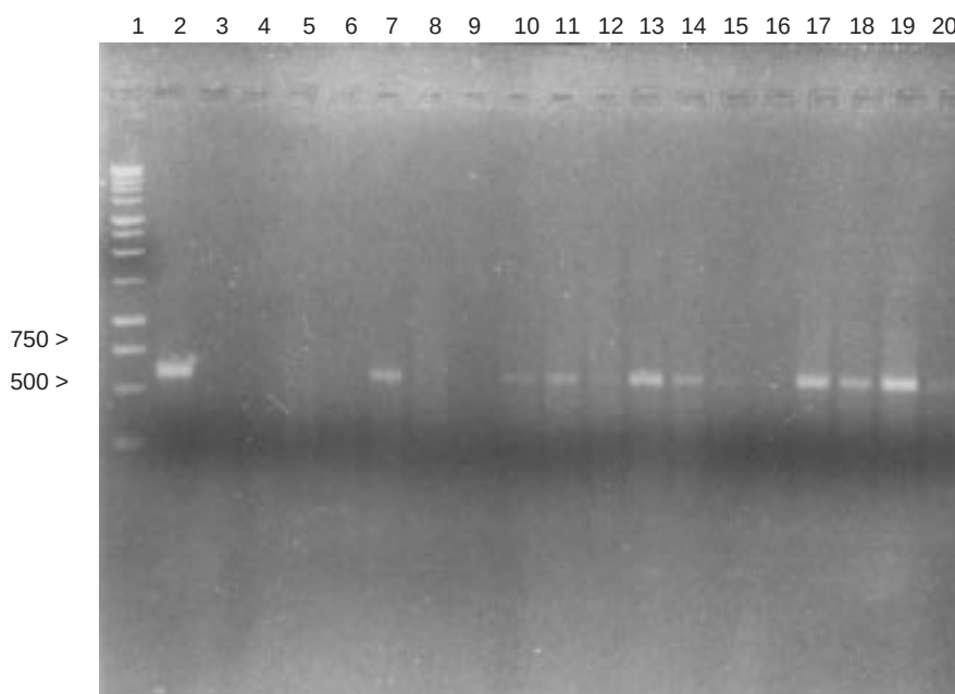
Figure 2. Detection of DNA from Fusarium oxysporum f.sp. ciceris in artificial soil by PCR using specific wilt-associated nested primers. DNA extracts were used for amplification at different stages during the extraction protocol: lanes 3–8, after treatment with skimmed milk solution and centrifugation; lanes 9–14, after deproteinisation; lanes 15–20, after DNA ethanol precipitation. Three different concentrations of skimmed milk solution were used with 1 µl of DNA extract for the amplification, either without dilution or after 10-fold dilution. Dilution occurred before amplification. Lanes: (3,9,15) 0.4% skimmed milk, no dilution; (4,10,16) 0.4% skimmed milk, 10-fold dilution; (5,11,17) 0.8% skimmed milk, no dilution; (6,12,18) 0.8% skimmed milk, 10-fold dilution; (7,13,19) 1.6% skimmed milk, no dilution; (8,14,20) 1.6% skimmed milk, 10-fold dilution. Lane (1) 1 kb ladder (Promega); Lane (2) positive control.
