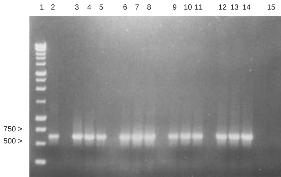
Figure 5. Detection of DNA from Fusarium oxysporum f.sp. ciceris DNA by PCR in one artificial and three natural soils using specific, wilt-associated, nested primers. The PCR was made using a modified 'touch down' for the annealing step. Three concentrations of skimmed milk were used. Lanes: (1) 1 kb ladder (Promega); (2) positive control; (3–5) artificial soil; (6–8) natural soil A; (9–11) natural soil C; (12–14) natural soil B; (3,6,9,12) 3.2% skimmed milk; (4,7,10,13) 4.0% skimmed milk; (5,8,11,14) 4.8% skimmed milk.
